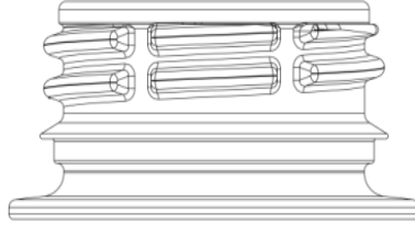
Neck - PCO 1873 28mm
