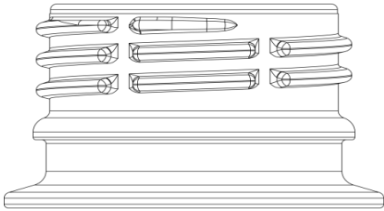
Neck - PCO 1816 28mm
