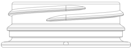
Neck- Heat Resistant 33mm – 2 strings 38 mm – 2 strings
